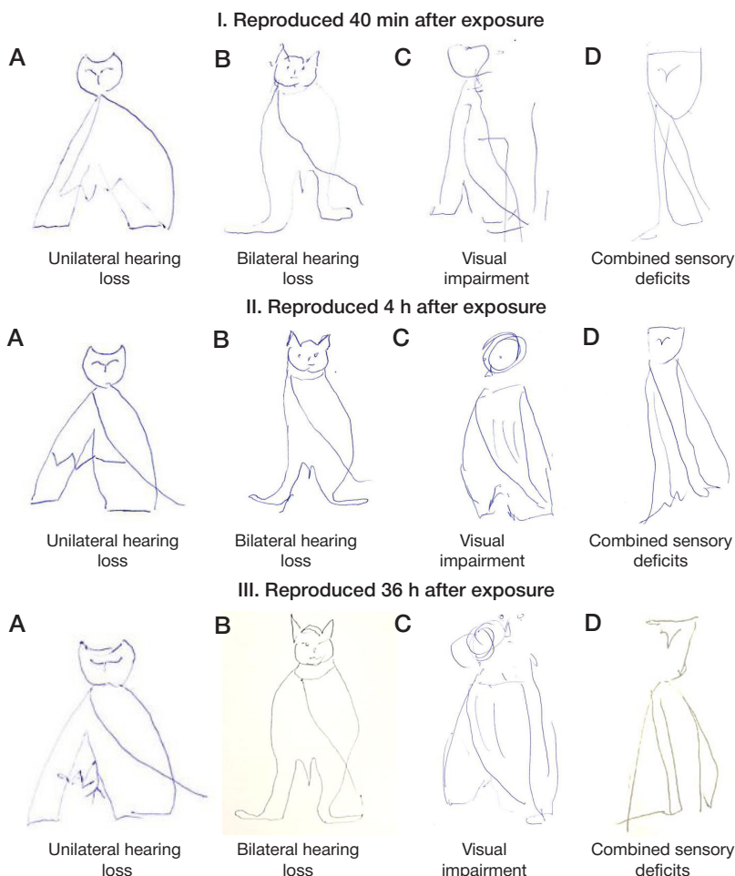
Fig. 3. Representative copies of the stimulus image made at different time points after exposure (40 min, 4 h, and 36 h) in four groups of the study
