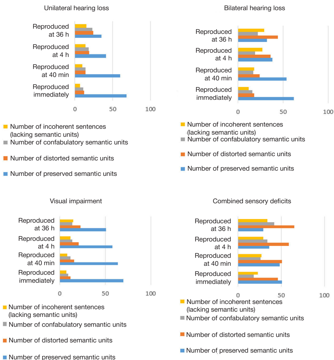
Fig. 5. Histograms of mean values for auditory-verbal memory indicators in four groups of the study
